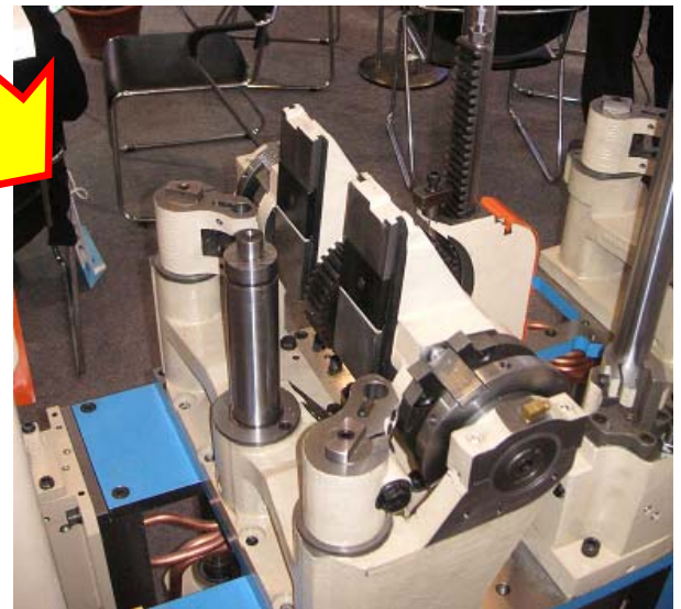
NECKRING MECH. & CC INVERT MECH.
